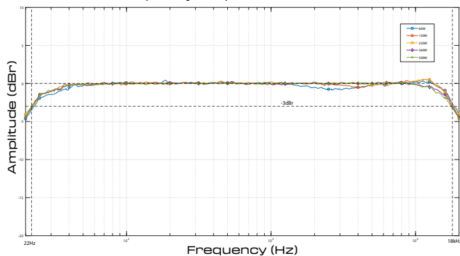
Frequency Response of MA3000 Series
